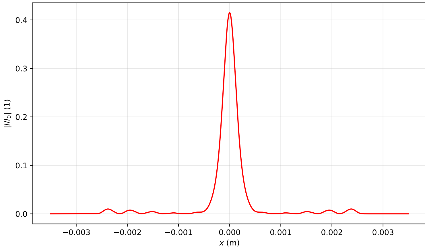
Intensity profile I(x, y = 0, z = 2.707)/I_0 , P_{in}=8.0P_{cr} , artificial time
